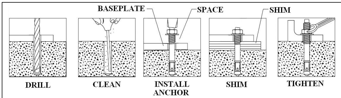
Figure 12. Anchor installation
