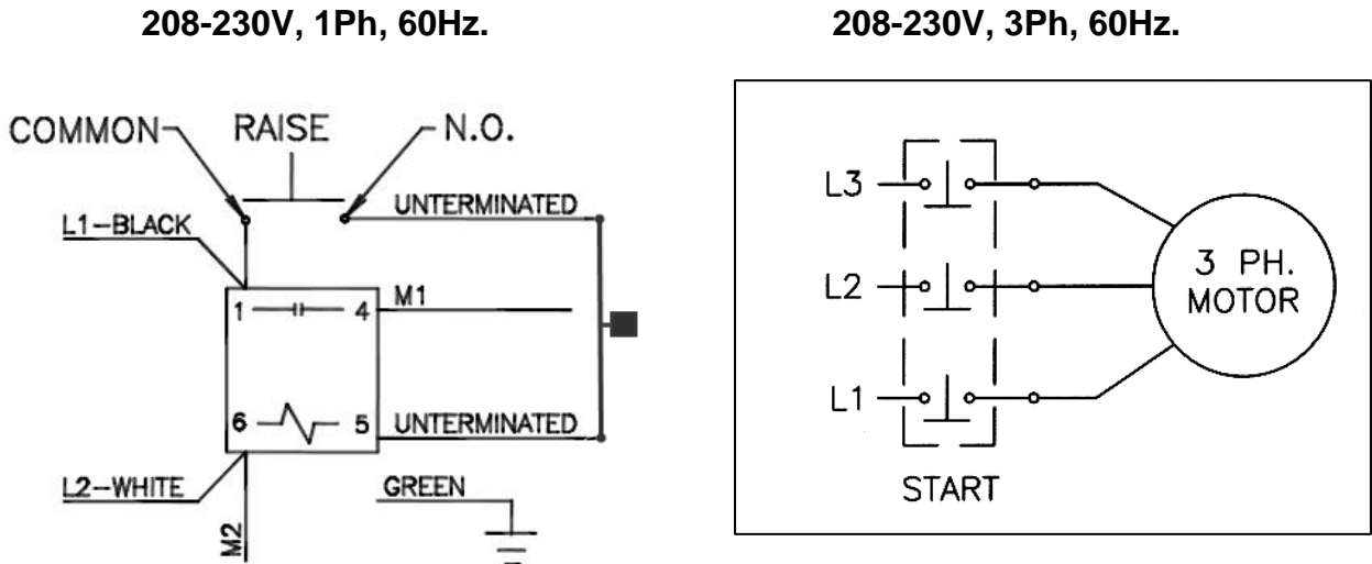
Figure 7. Electrical diagram for 230V/1 Ph and 230V/3 Ph
